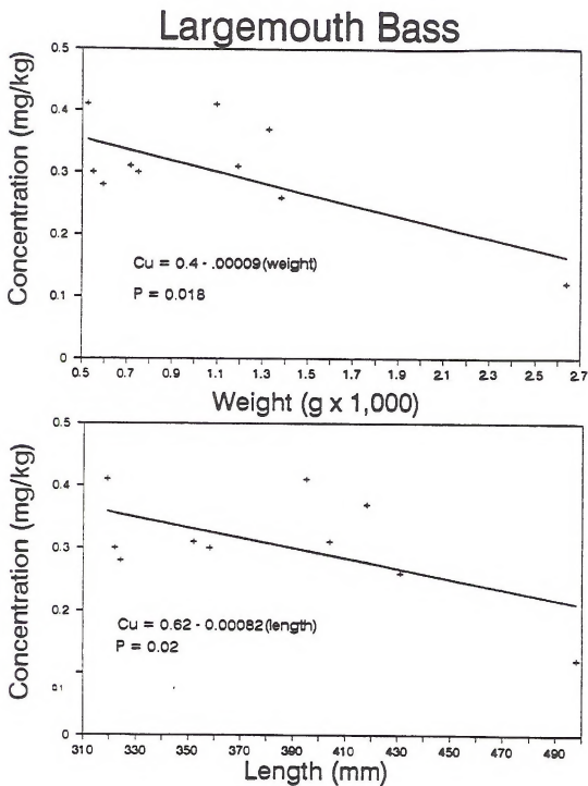
Figure 7. Linear relationships between concentration of copper in largemouth bass flesh as a function of body size.
